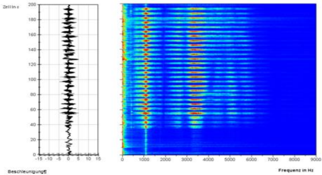
Figure 13 Time versus acceleration and time versus frequencies during jet grouting against a primary column
