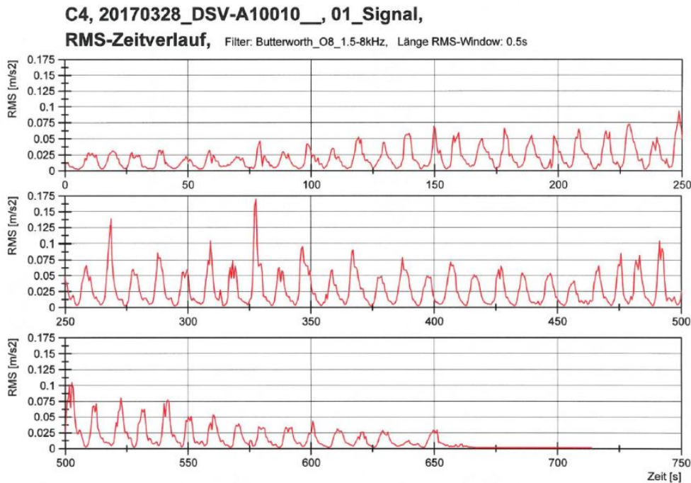
Figure 17: Production process of column C4
