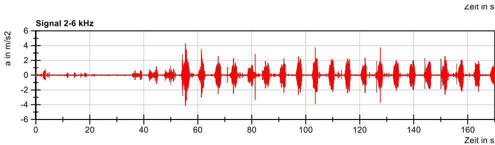
Figure 14: Processed signals by bandpass filter ( 2-6 kHz)
