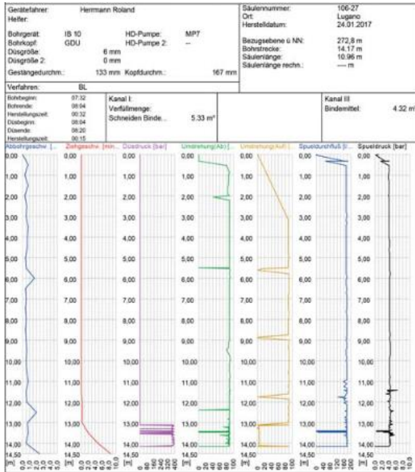
Figure 6 Recording of execution parameters (source: internet presentation Fa. Bauer )
