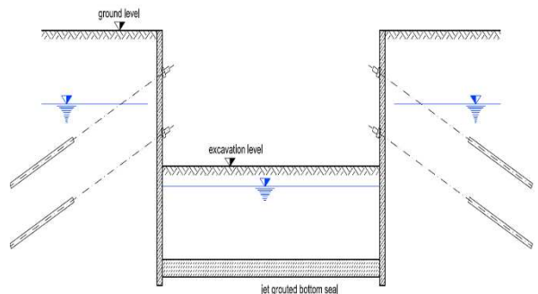
Figure 4 Bottom sealed excavation pit
